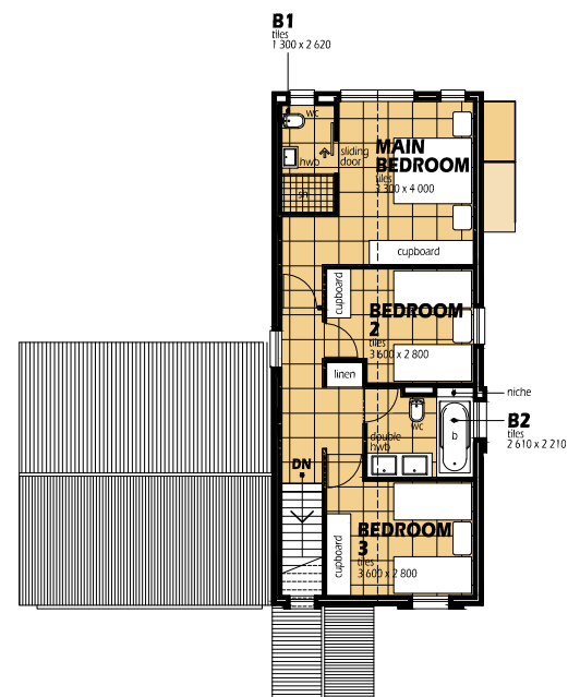
FIRST FLOOR LAYOUT
