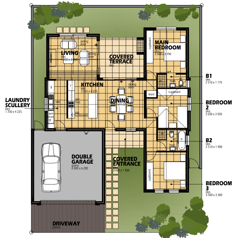
FLOOR LAYOUT
