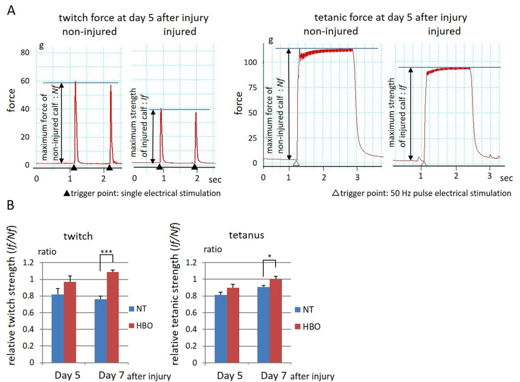
Figure 4. HBO increased the isometric tensile strength of the gastrocnemius muscle. (A) Twitch and tetanic forces were recorded and ratios of injured leg ( If ) to non-injured leg forces ( Nf ) were calculated. (B) The ratio of twitch muscle strength in the HBO group was higher than that in the NT group at 7 days. The maximum strength of tetanic forces in the HBO group was higher than that in the NT group at 7 days. n = 6 . *** P < 0.001 , * P < 0.05 using Student's t test. Data are the mean \pm SEM.
