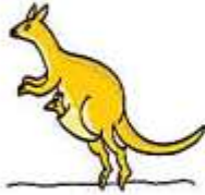
kangaroo
