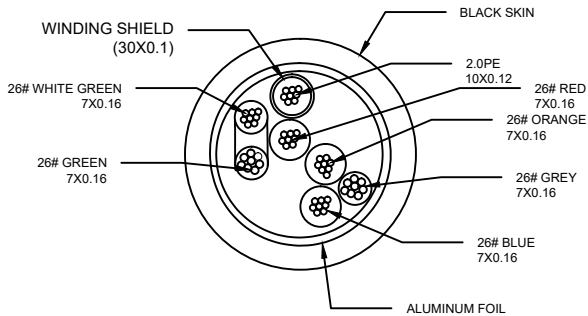
X-X WIRE SECTION
