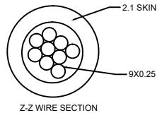
Z-Z WIRE SECTION
