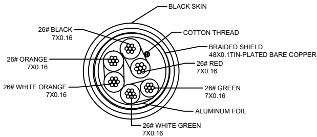
Y-Y WIRE SECTION
