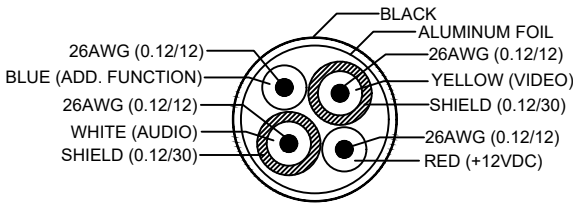
SECTION Z-Z
