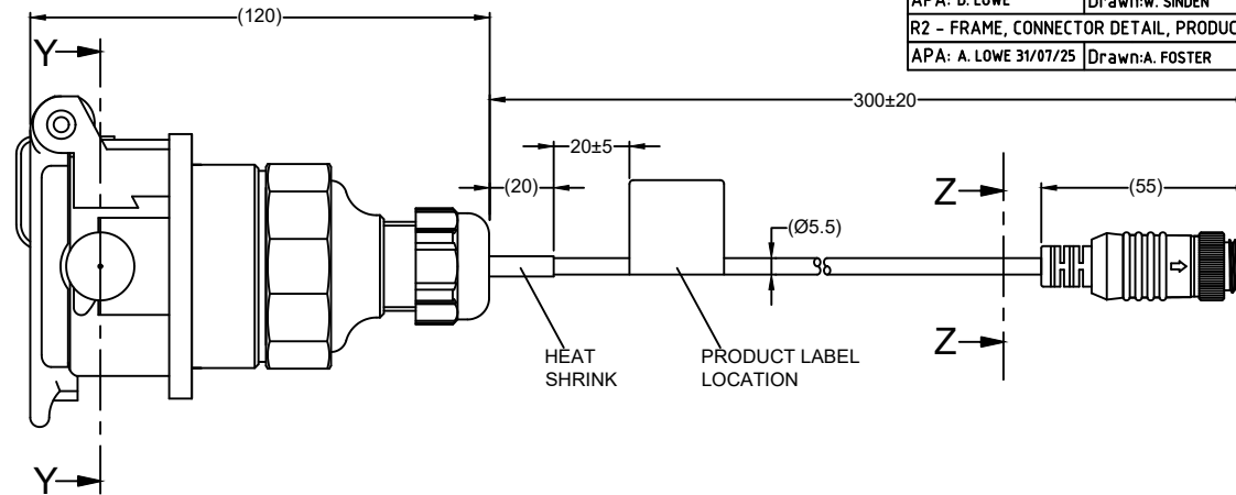
SECTION Z-Z
