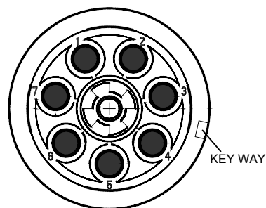
7 PIN MALE MATING FACE
