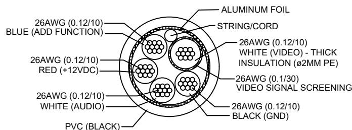
CABLE BUILDUP
