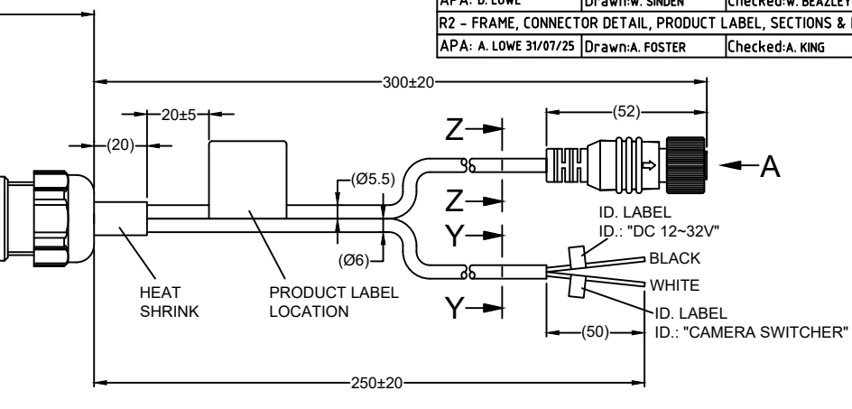
SECTION Z-Z
