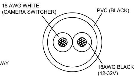
CABLE BUILDUP
