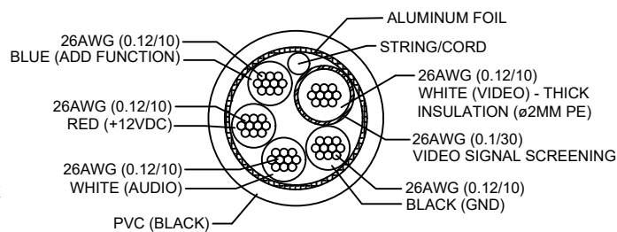
CABLE BUILDUP
