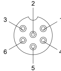
6 PIN FEMALE MATING FACE
